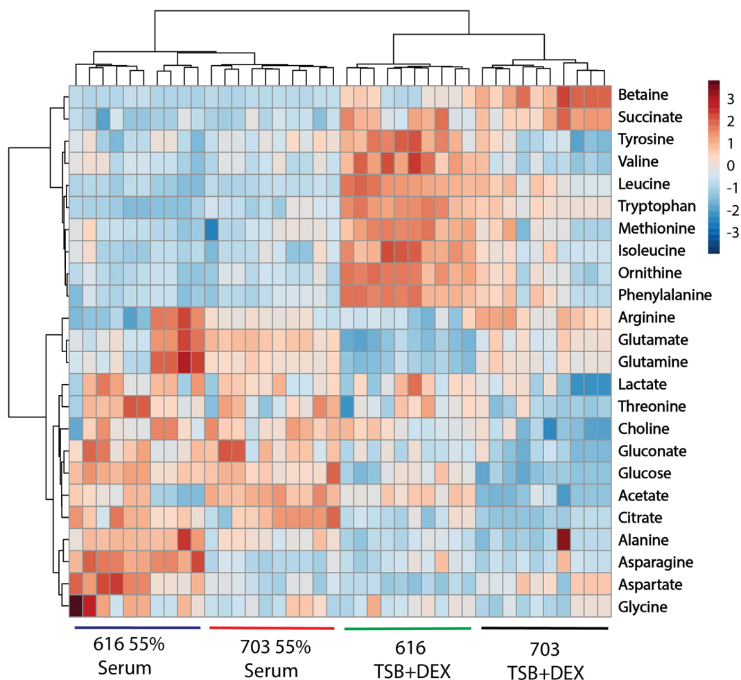
Figure 4. Heatmap and hierarchal clustering highlighting the metabolic alterations of S. aureus strains 616 and 703 due to the presence of 55% serum. The heat map plots normalized peak intensities from the 2D ^1\text{H} - ^{13}\text{C} HSQC spectra. Each row displays the relative metabolite abundance for each replicate from the four groups, where red identifies a relative increase and blue indicates a relative decrease in the metabolite. Note all replicates per group cluster together.
