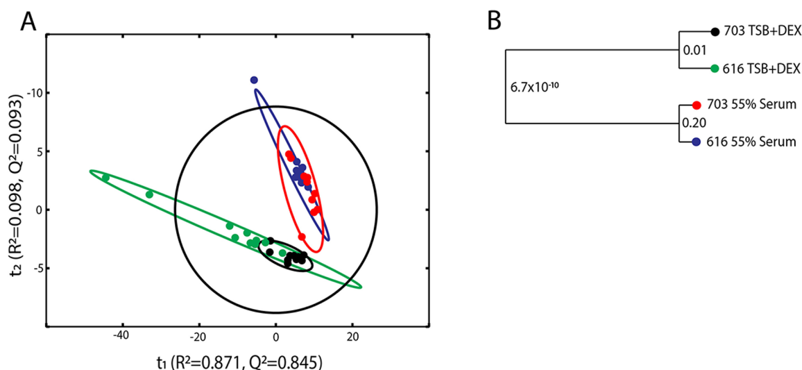
Figure 3. Statistical analysis of 1D 1 H NMR data set obtained from S. aureus strains 616 and 703 in the presence and absence of 55% serum. (A) PCA scores plot comparing the metabolomes from S. aureus strains 616 and 703 in TSB+DEX (green, black) and in 55% serum (blue, red). The R 2 and Q 2 are 0.981 and 0.938, respectively. (B) A dendrogram generated from the PCA model in A where each node is labeled with a p -value. The ellipses in the PCA scores plot represent the 95% confidence limit of the normal distribution for each group.
